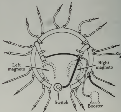
FIGURE 4-11. Accessory-mounted, nine-cylinder engine ignition harness.
